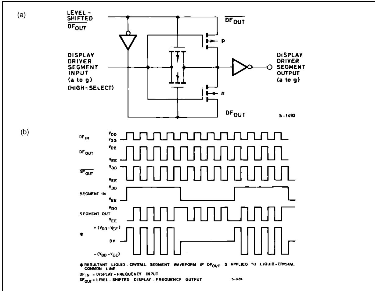
Figure 10 : Clock Display.
