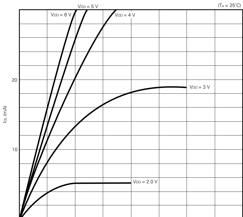
I OL vs V OL (Port 3, 4, and 5)
