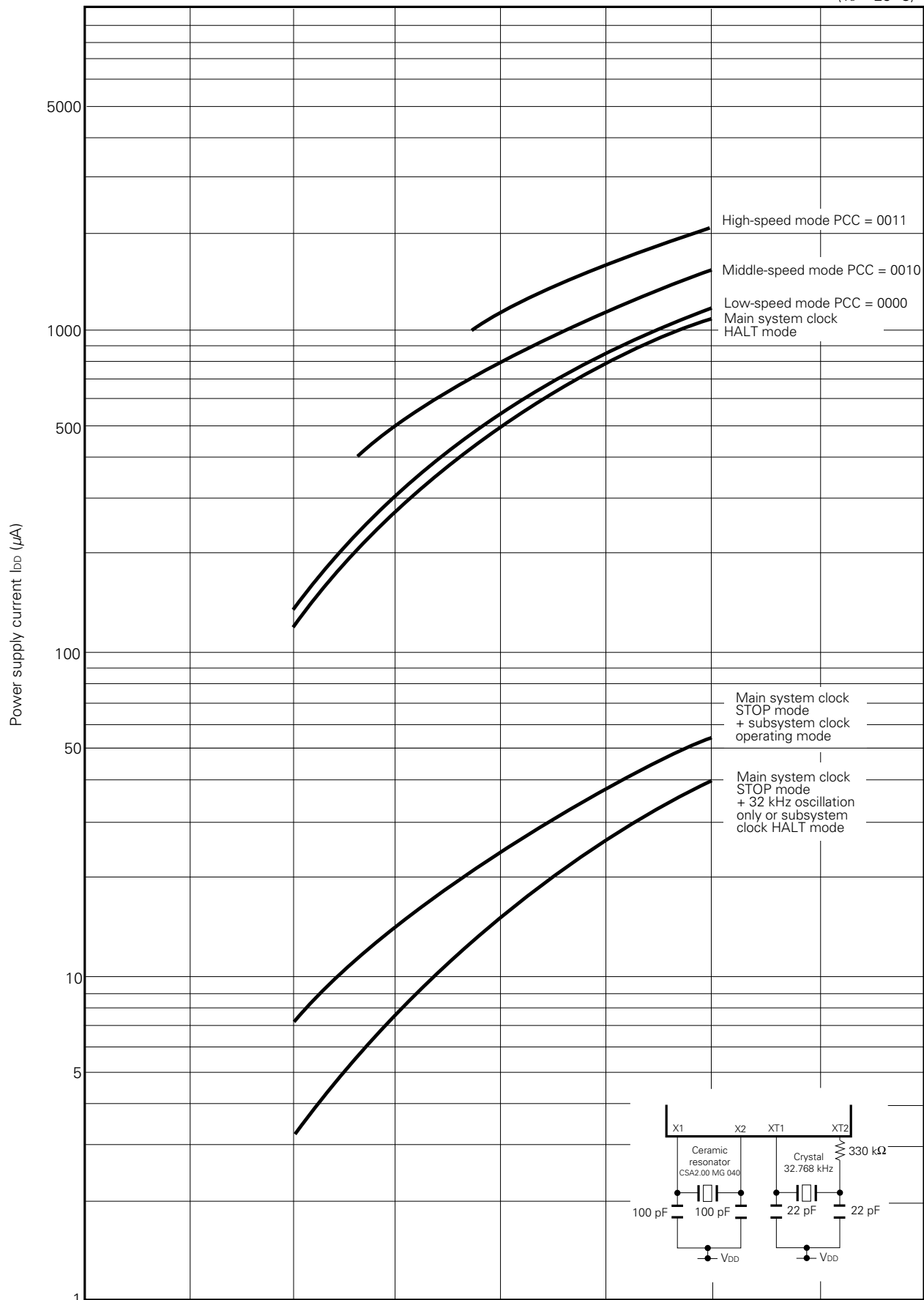
I_{DD} vs V_{DD} (Ceramic Oscillation: 2.00 MHz)
