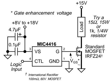
Figure 1. Using a Standard MOSFET
