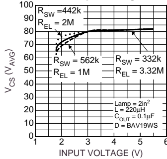
CS Voltage vs. Input Voltage
