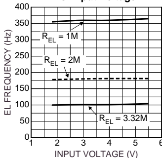
EL Frequency vs. Input Voltage
