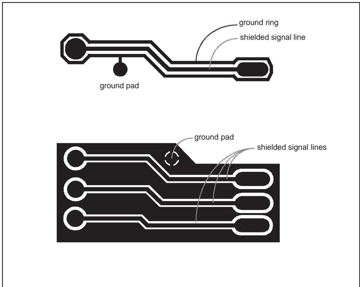
Figure 6-8. Shielding signals
