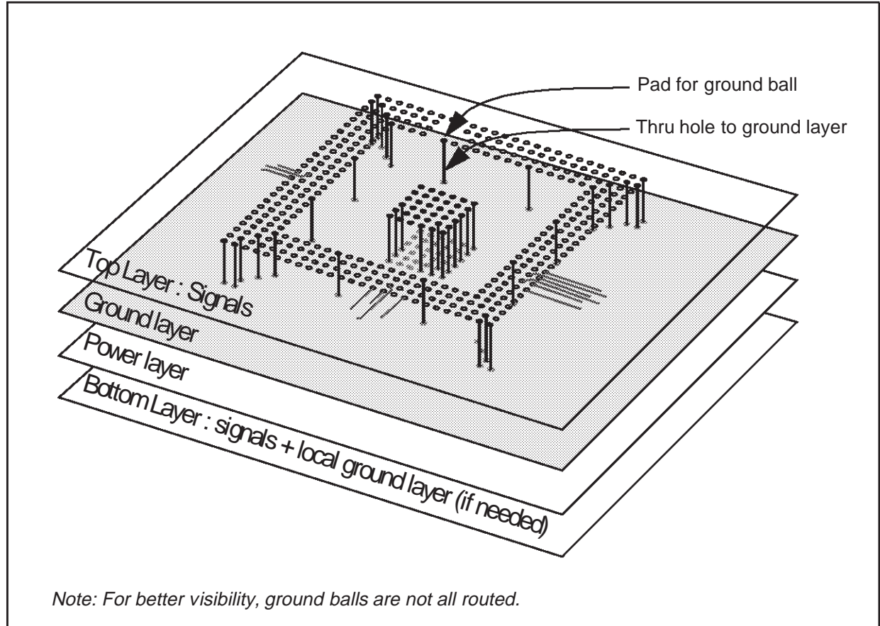
Figure 6-1. Ground routing
