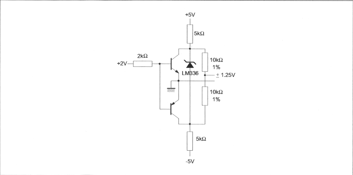
Figure 8 : Bipolar Output Reference
