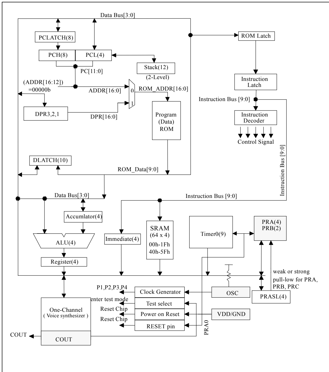
FIGURE 1.1 : Block Diagram of ASM3106C
