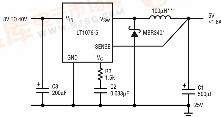
Basic Positive Buck Converter
