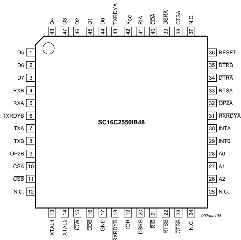
Fig 4. LQFP48 pin configuration.
