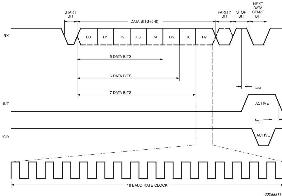
Fig 11. Receive timing.
