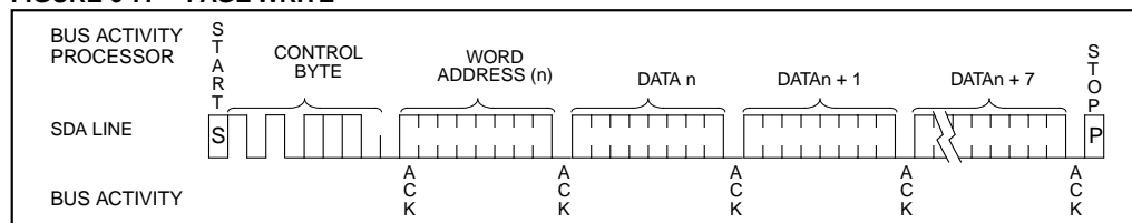
FIGURE 6-7: PAGE WRITE
