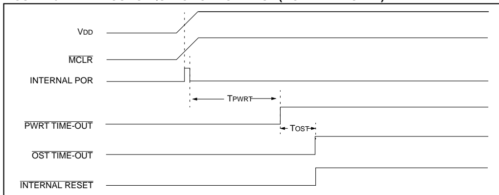
FIGURE 10-11: TIME-OUT SEQUENCE ON POWER-UP (MCLR TIED TO V DD )
