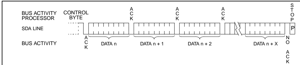
FIGURE 6-10: SEQUENTIAL READ
