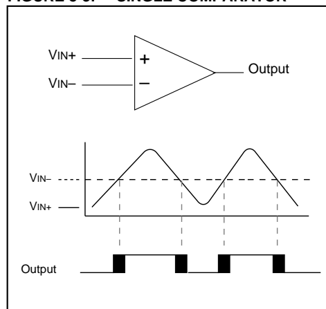
FIGURE 8-3: SINGLE COMPARATOR
