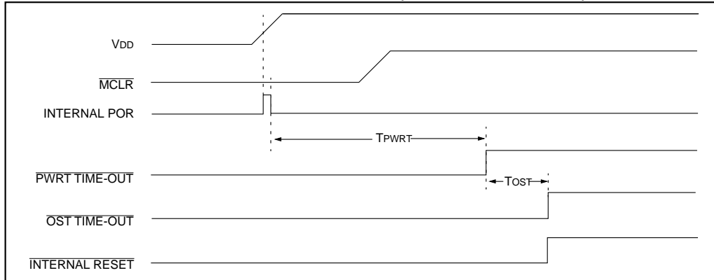
FIGURE 10-10: TIME-OUT SEQUENCE ON POWER-UP (MCLR NOT TIED TO V DD ): CASE 2
