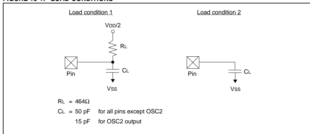
FIGURE 13-1: LOAD CONDITIONS
