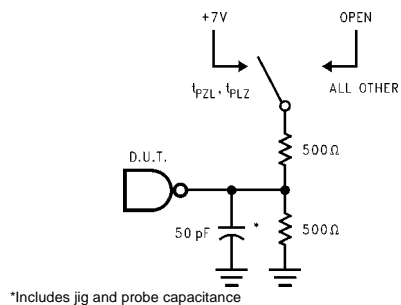
FIGURE 5. Standard AC Test Load
