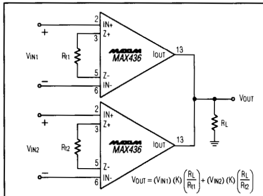
Figure 7. Summing Amplifier
