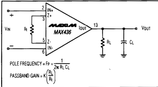
Figure 8. Lowpass Amplifier
