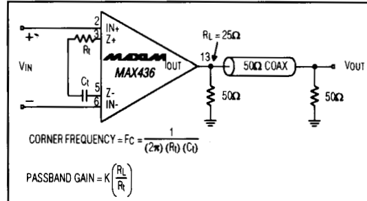
Figure 10. Highpass Amplifier
