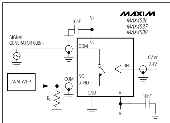
Figure 4. Off Isolation
