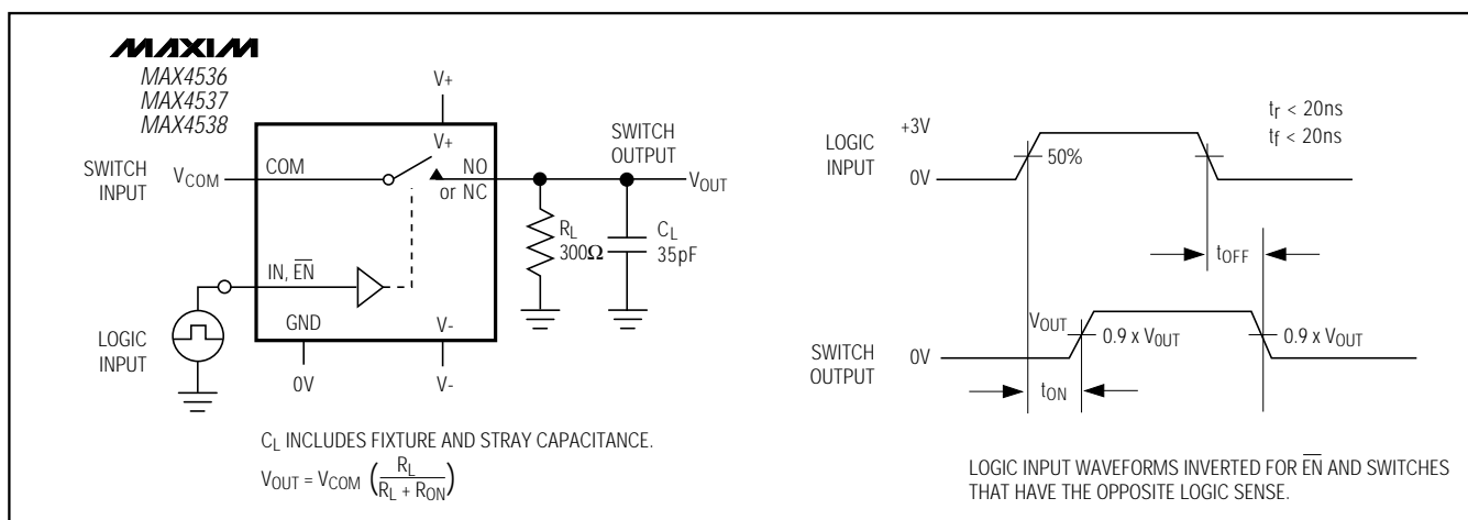
Figure 1. Switching Time
