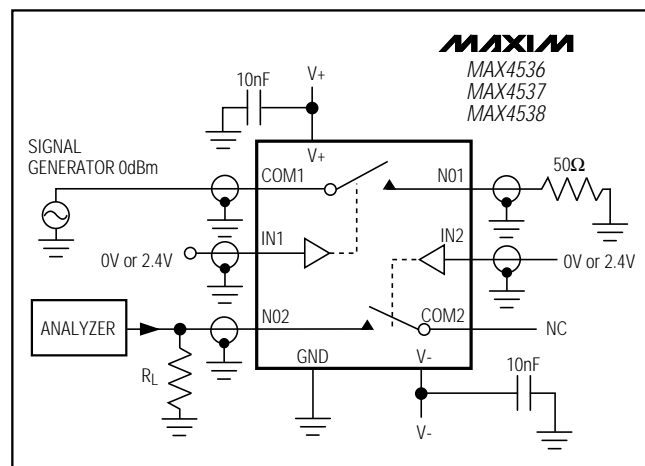
Figure 5. Crosstalk
