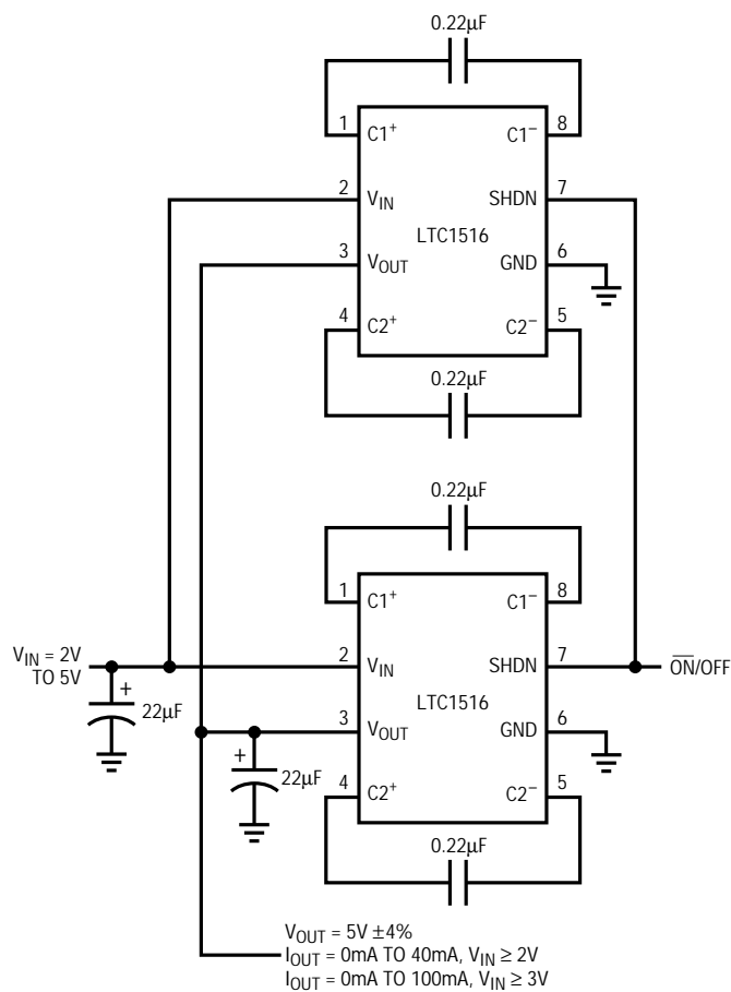
Figure 5. Paralleling Devices
