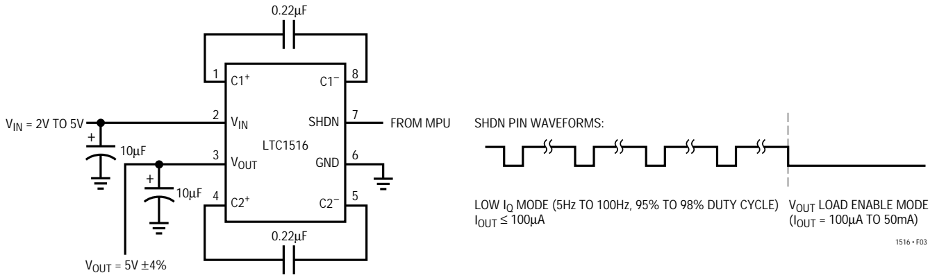
Figure 3. Ultralow Quiescent Current ( <5\mu\text{A} ) Regulated Supply
