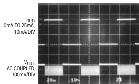
Load Transient Response, V_{IN} = 3\text{V}
