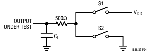
Figure 4. Driver Timing Test Load #2
