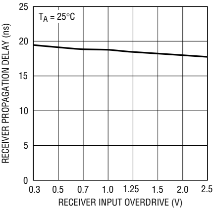
Receiver Propagation Delay vs Input Overdrive
