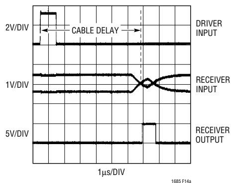
Figure 14a. 4000 Feet of Category 5 UTP 1μs Pulse
