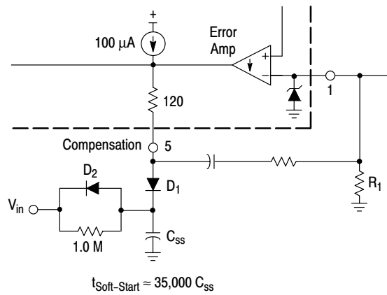
Figure 18. Soft-Start Circuit
