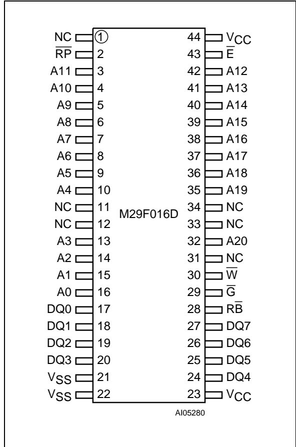
Figure 4. SO Connections
