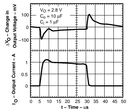
TPS72618 LOAD TRANSIENT RESPONSE
