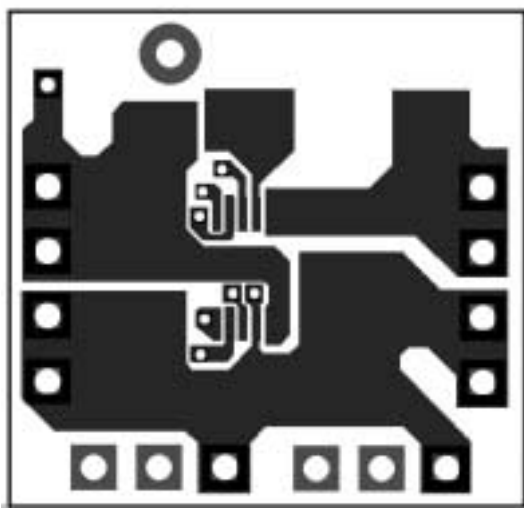
Figure 20. Top Layer Layout and Component Placement
