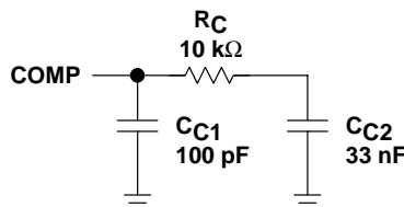
Figure 19. Compensation of the Control Loop
