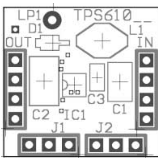
Figure 20. Top Layer Layout and Component Placement
