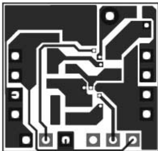
Figure 21. Bottom Layer Layout and Component Placement
