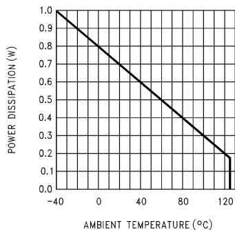
Maximum Power Dissipation (TO-92)
