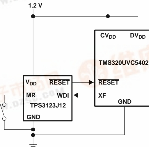
Figure 1. Typical Low-Voltage DSP Application
