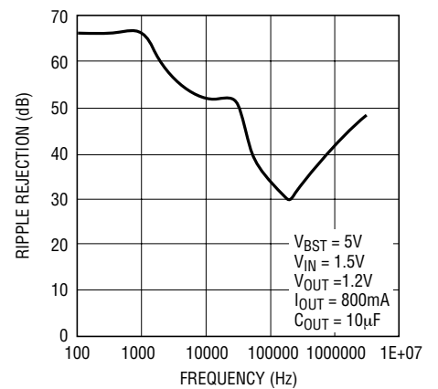
Ripple Rejection
