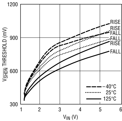
Shutdown Threshold
