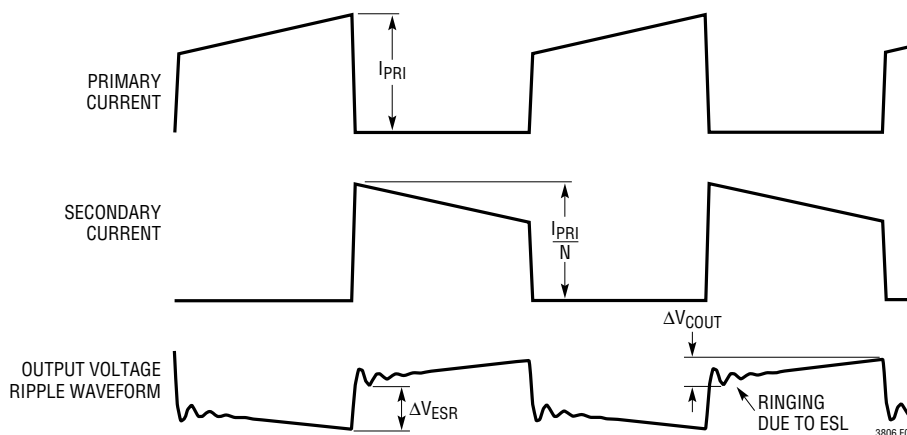
Figure 5. Typical Flyback Converter Waveforms (Single Output)
