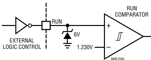
Figure 3b. On/Off Control Using External Logic
