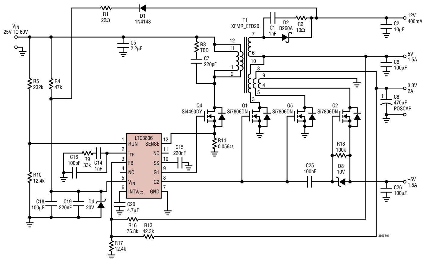
Figure 7. Synchronous Flyback
