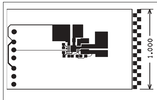
SP6656 PC Layout Top Side
