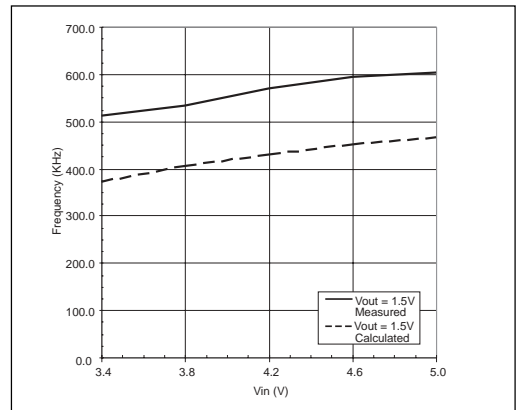
Ripple Frequency vs. V_{IN} , I_{OUT}=0.4A , V_{OUT}=1.5V
