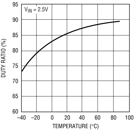
Maximum Duty Ratio
