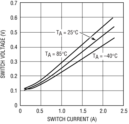
Switch Saturation Voltage vs Current
