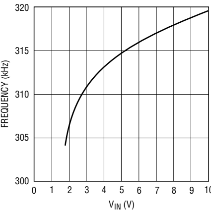
Oscillator Frequency Line Regulation
