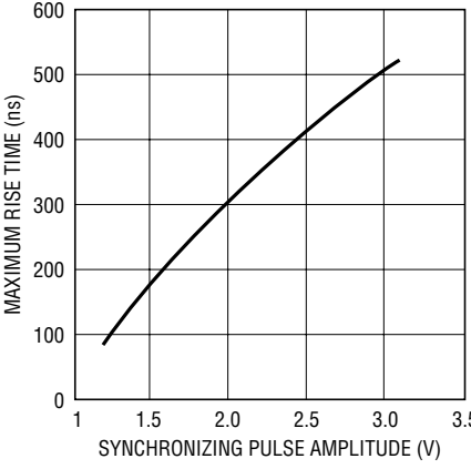
Maximum Allowable Rise Time of Synchronizing Pulse
