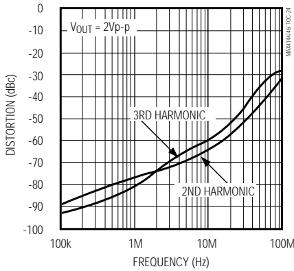
MAX4146 HARMONIC DISTORTION vs. FREQUENCY ( A_V = +100 )
