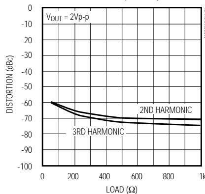
MAX4146 5MHz HARMONIC DISTORTION vs. LOAD ( A_V = +100 )
