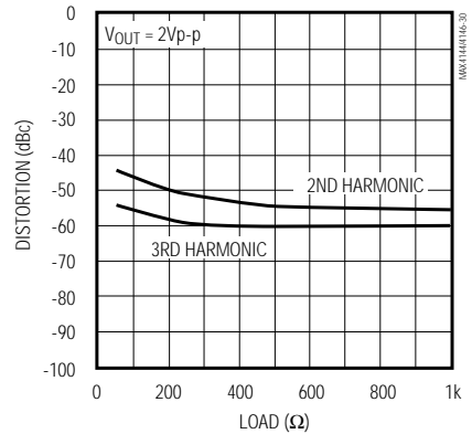
MAX4146 5MHz HARMONIC DISTORTION vs. LOAD ( A_V = +10 )
