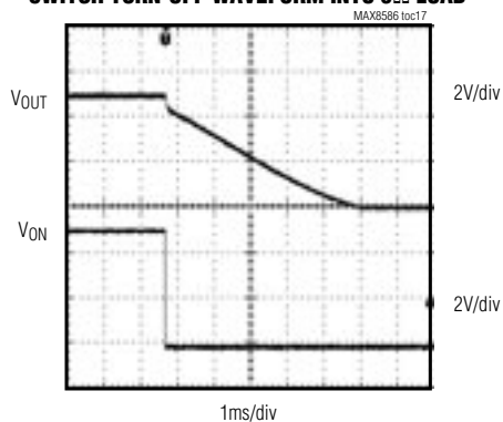
SWITCH TURN-OFF WAVEFORM INTO 5\Omega LOAD
