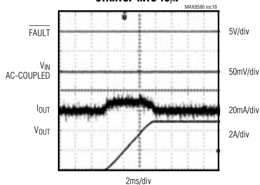
STARTUP INTO 10\mu F
