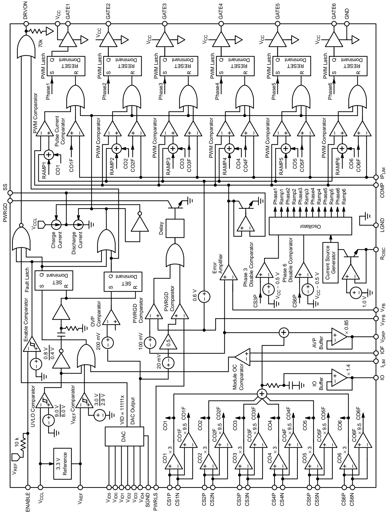
Figure 3. Block Diagram
