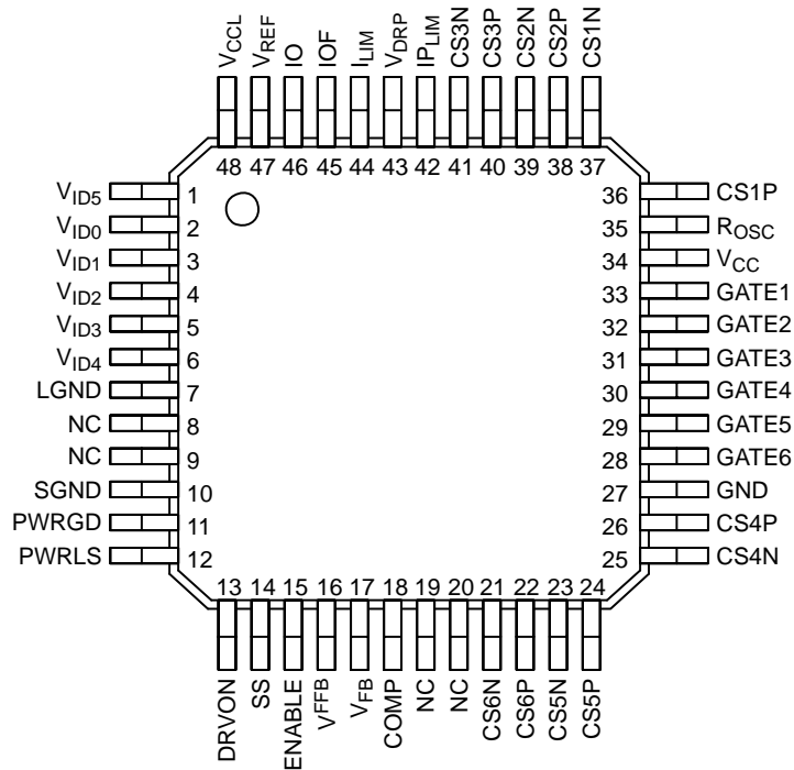
LQFP-48
