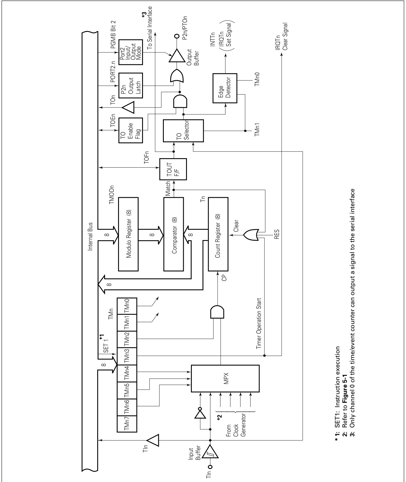
Figure 5-4 Block Diagram of Timer/Event Counter (n=0, 1)
