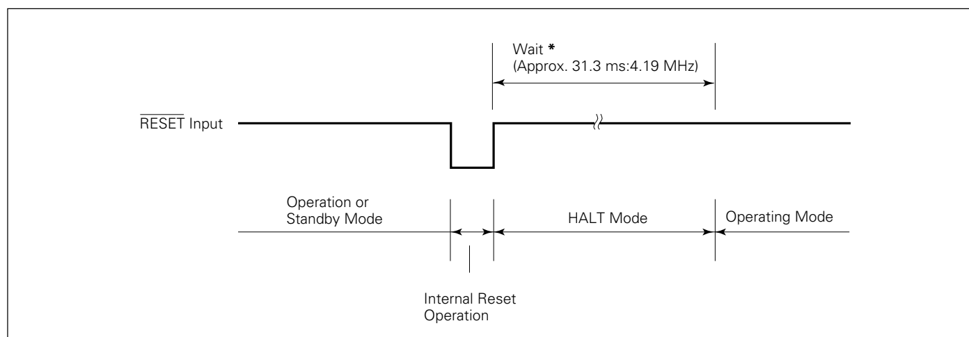
Figure 8-3 Reset Operation by Reset Input
