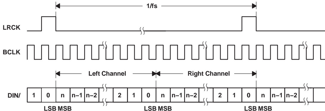
Figure 12. Timing Diagram for DSP Mode
