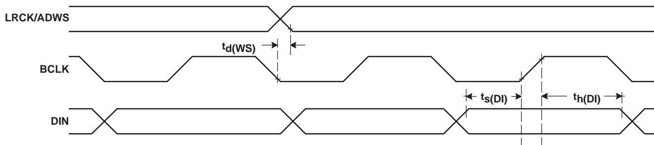
Figure 1. I²S/LJF/RJF Timing in Master Mode
