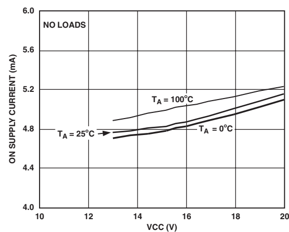
TPC 6. ON Supply Current vs. VCC
