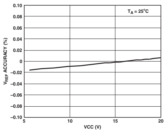
TPC 5. V_{REF} Accuracy vs. VCC
