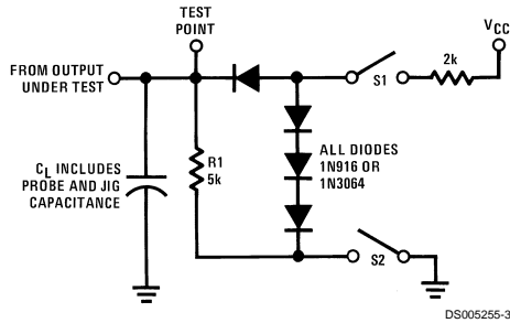
Load Test Circuit for TRI-STATE® Outputs
