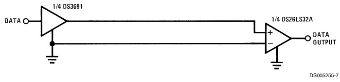
Single Wire with Driver Ground Reference—RS-423
