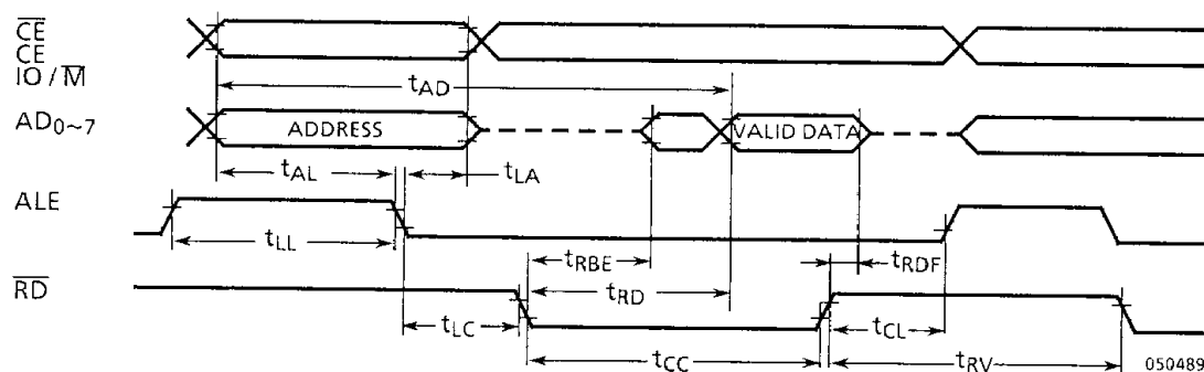
Figure 8.1 READ CYCLE
