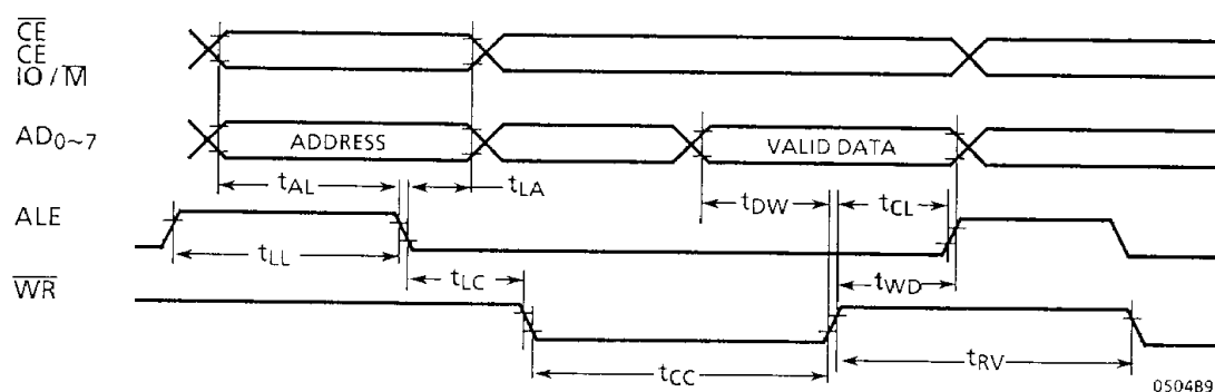
Figure 8.2 WRITE CYCLE
