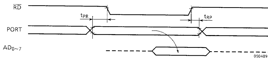
Figure 8.3 BASIC INPUT MODE
