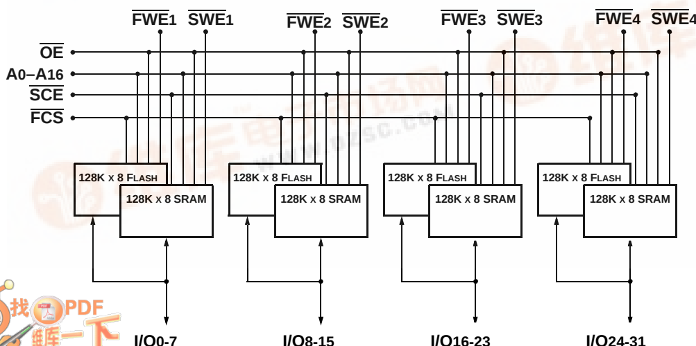
Block Diagram – PGA Type Package (P3 & P7)
