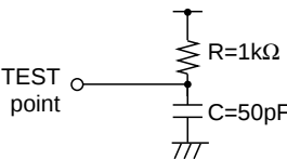
Figure 5 Timing Load
