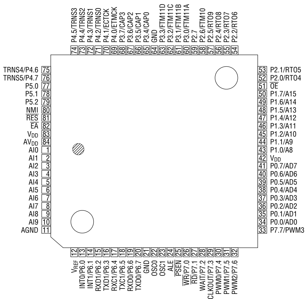
84-Pin Plastic QFJ (PLCC)
