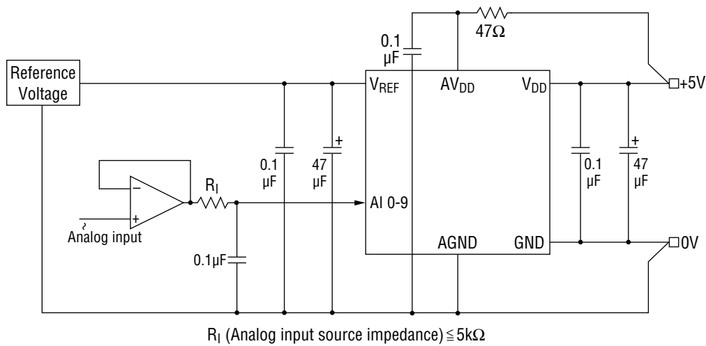
Figure 1 Recommended Circuit
