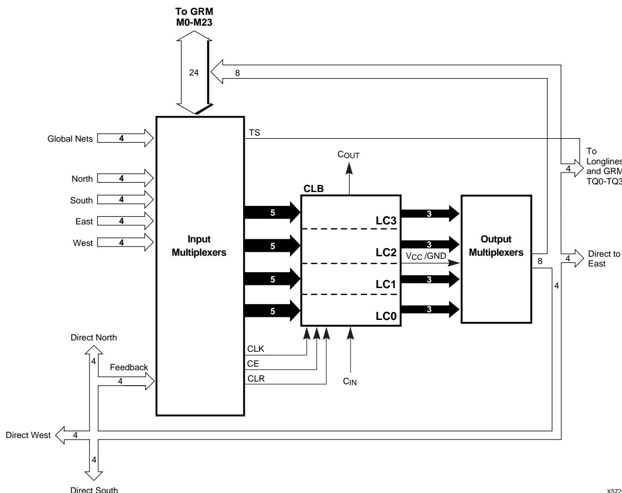
Figure 14: VersaBlock Details
