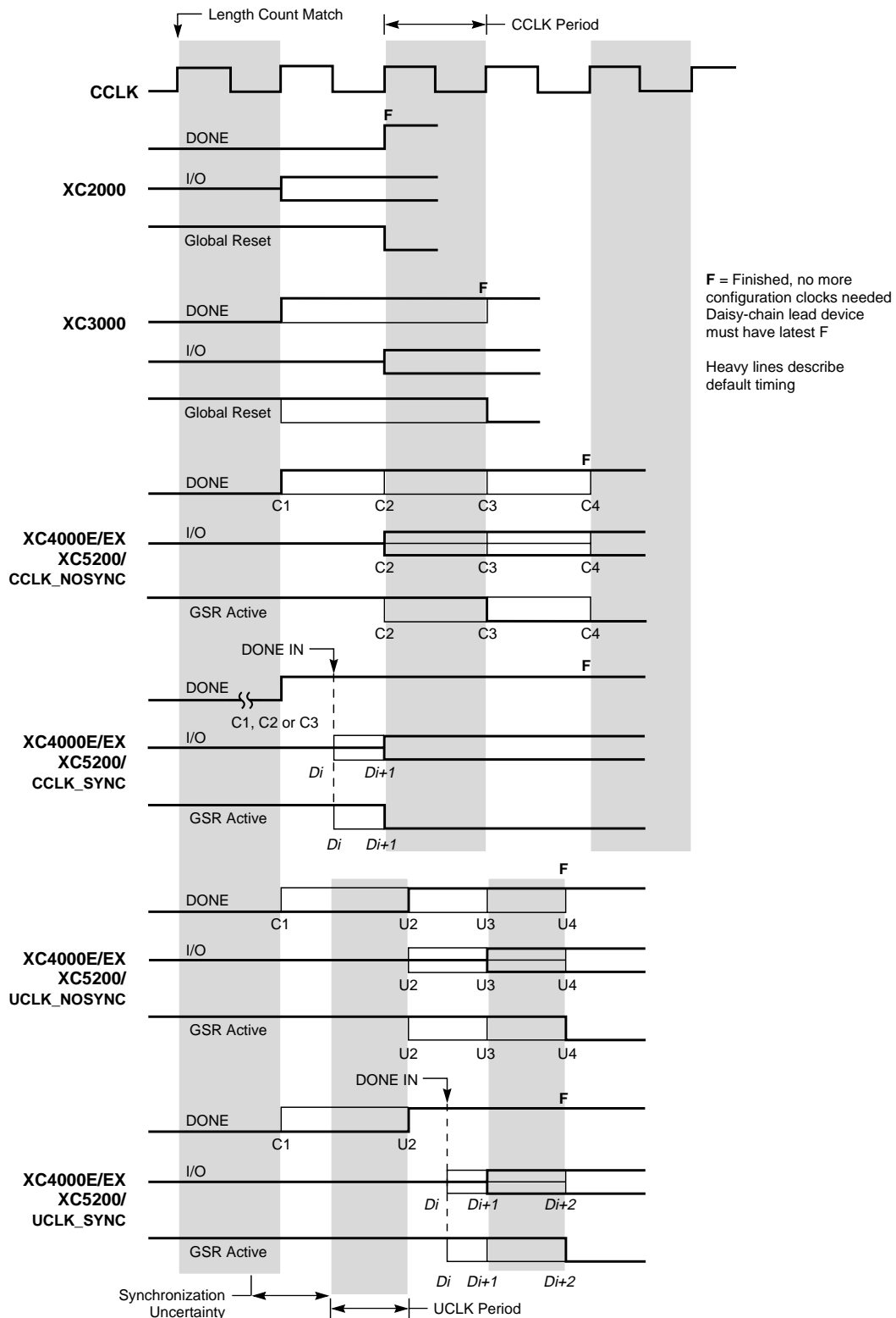
Figure 25: Start-up Timing
