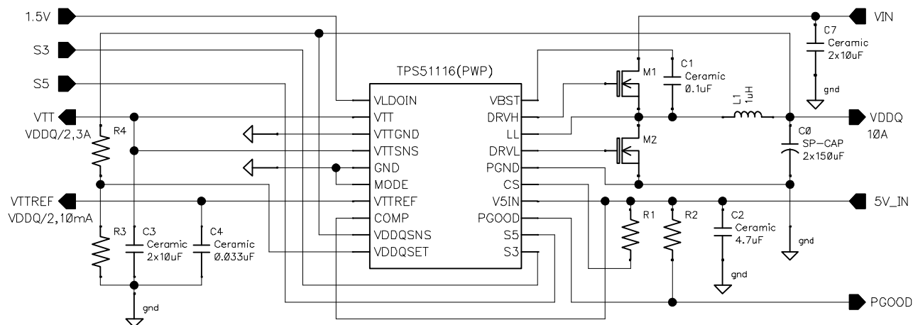
Figure 4. D-CAP™ Mode
