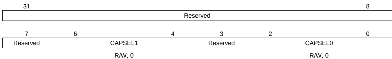
Figure 4-41. CFGRTI Register Bit Layout (0x4000 0014)
