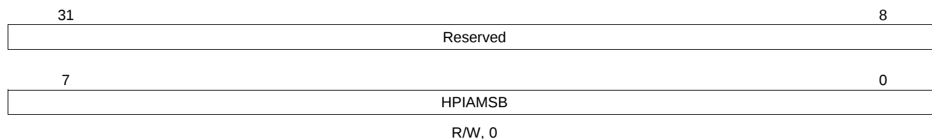
Figure 4-19. CFGHPIAMSB Register Bit Layout (0x4000 000C)
