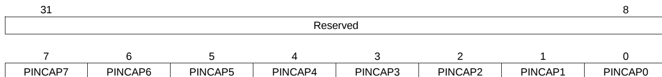
Figure 2-6. CFGPIN0 Register Bit Layout (0x4000 0000)
