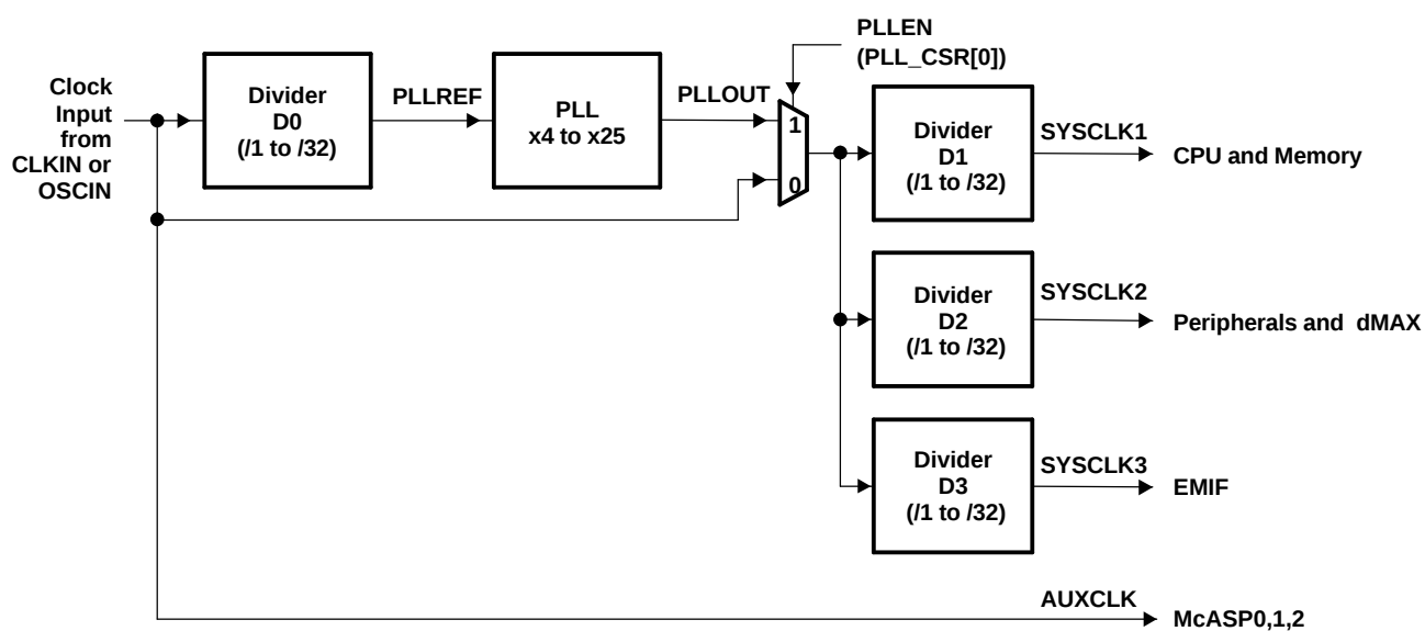
Figure 4-43. PLL Topology
