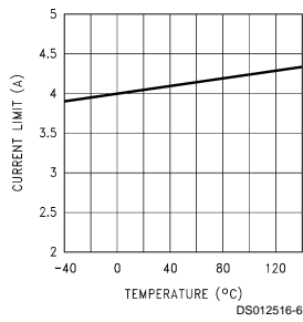
Current Limit vs Temperature
