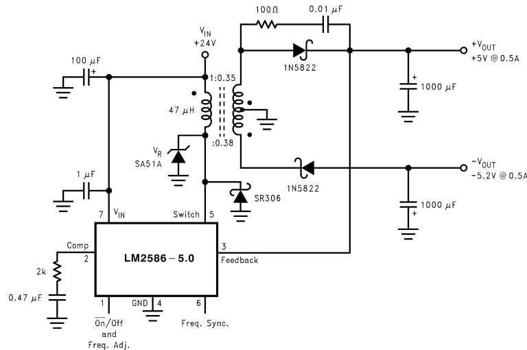
FIGURE 43. Flyback Regulator
