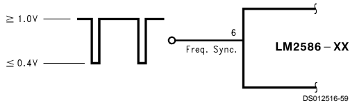
FIGURE 40. Frequency Synchronization
