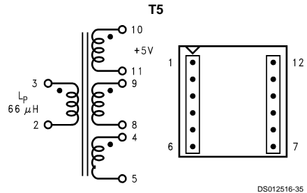
FIGURE 17. Coilcraft Q4437-B (Surface Mount)
