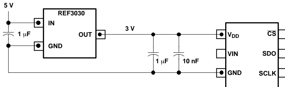
Figure 30. Using the REF3030 Reference
