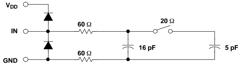
Figure 28. Typical Equivalent Sampling Circuit
