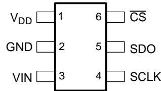
SOT23/SC70 PACKAGE (TOP VIEW)
