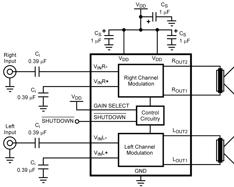
FIGURE 2. Single-Ended input with low gain selection configuration
