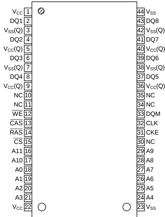
44-Pin Plastic TSOP (II) (K Type)
