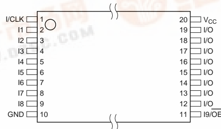
DIP/SOIC
