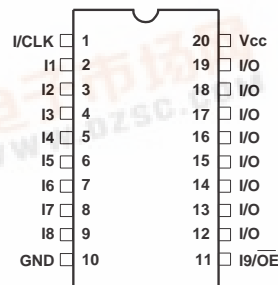
DIP/SOIC
