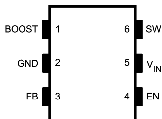
6-Lead TSOT NS Package Number MK06A
