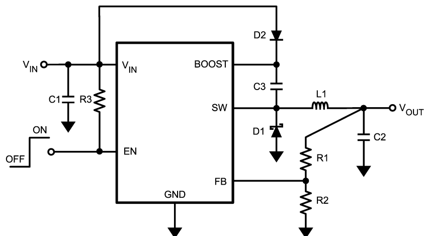
FIGURE 6. LM2736X (1.6MHz) V_{\text{BOOST}} Derived from V_{\text{IN}} 5V to 1.5V/750mA
