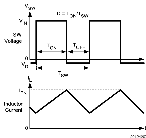
FIGURE 2. LM2736 Waveforms of SW Pin Voltage and Inductor Current
