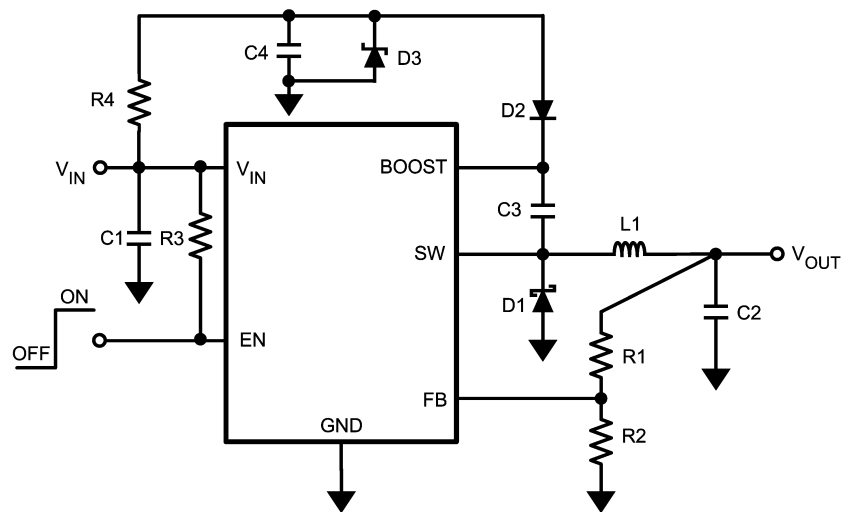
FIGURE 8. LM2736X (1.6MHz) V_{\text{BOOST}} Derived from V_{\text{SHUNT}} 18V to 1.5V/750mA
