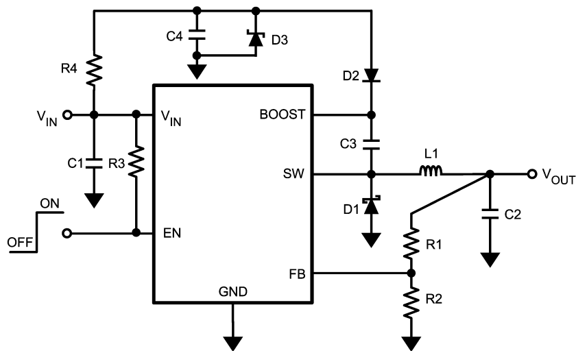
FIGURE 13. LM2736Y (550kHz) V_{\text{BOOST}} Derived from V_{\text{SHUNT}} 18V to 1.5V/750mA
