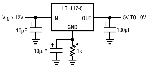
Adjusting Output Voltage of Fixed Regulators
