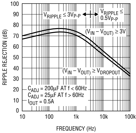
LT1117 Ripple Rejection
