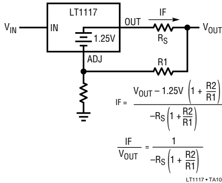
Battery Charger
