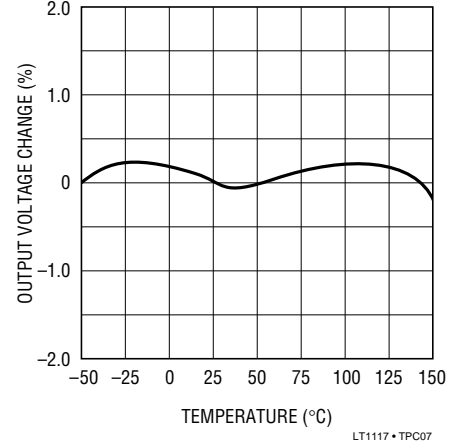
Temperature Stability
