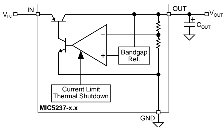
Fixed Regulator
