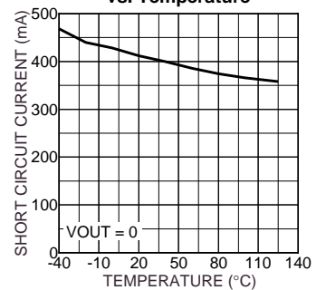
Short Circuit Current vs. Temperature
