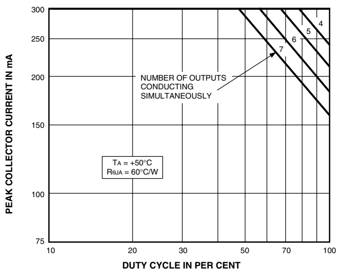
ULN7003A at T_A = +50^\circ\text{C}
