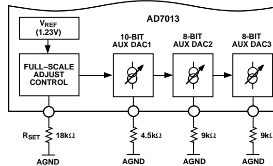
Figure 22. AUX DACs
